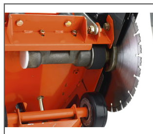
OPTIMAL POWER TRANSMISSION TO THE BLADE Enhanced belt tensioning system gives constant tension without need of re-tensioning, ensuring optimal performance and increased belt life.
