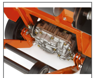
SELF-CONTAINED DRIVE SYSTEM Self-contained differential drive system eliminating drive gear from rear wheels and related wear. It is simple to handle and maintain.
